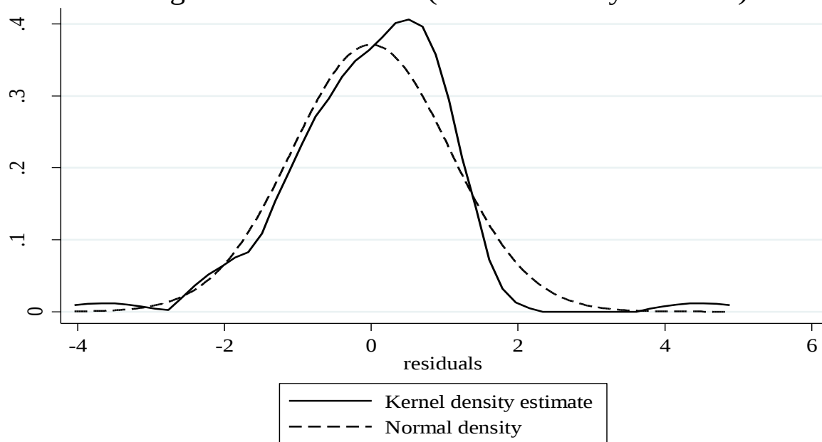
Figure A11: Model 11 (Kernel Density Estimate)
