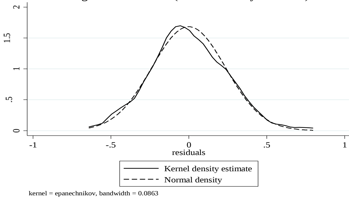
Figure A2 Model 2 (Kernel Density Estimate)
