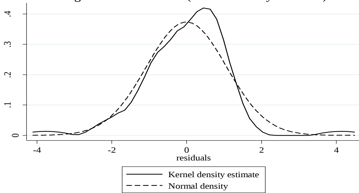
Figure A12: Model 12 (Kernel Density Estimate)
