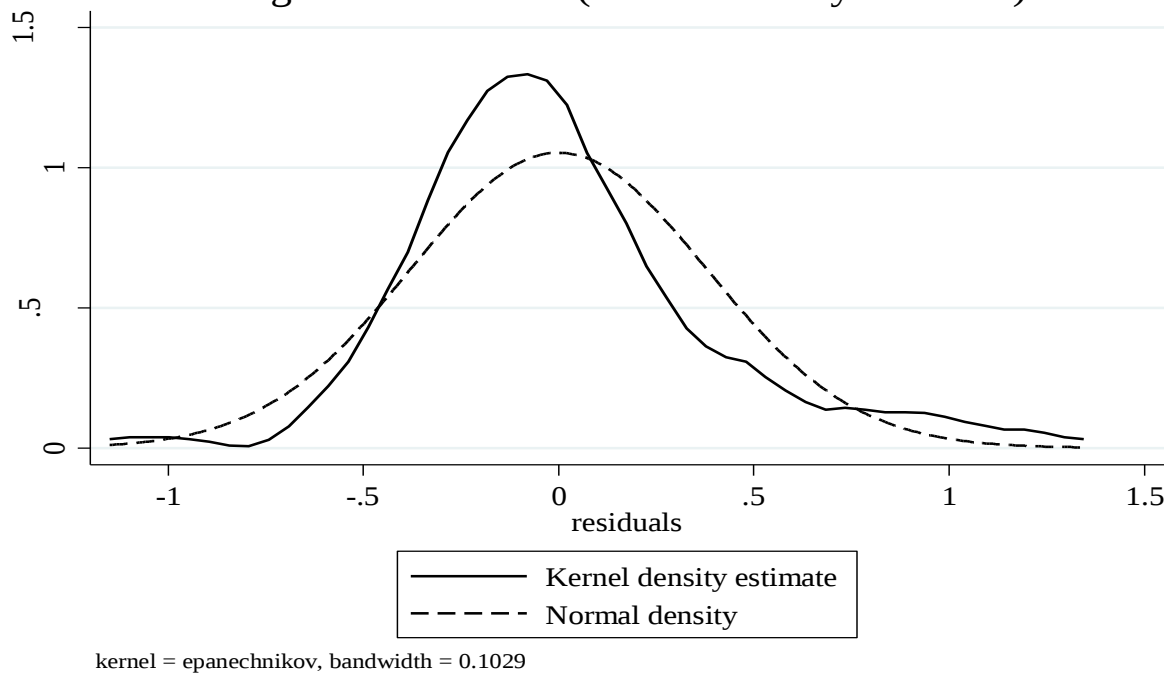
Figure A3 Model 3 (Kernel Density Estimate)
