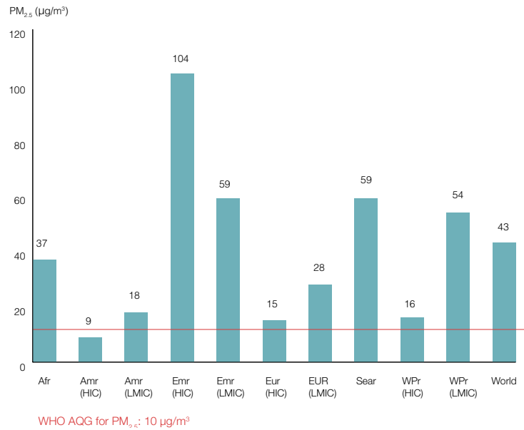
Figure 11: Annual median exposure to ambient (outdoor) PM 2.5 in µg/m 3 , by region - urban population only, 2014
