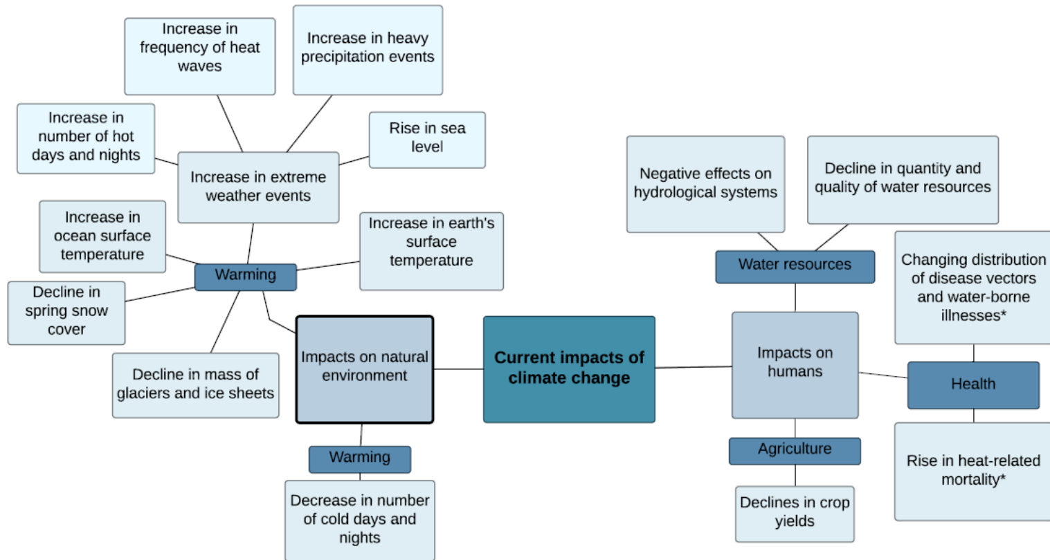
Figure 2.1 Current impacts of climate change on human and natural systems
