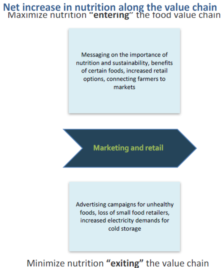
Figure 6.5 Climate change and nutrition entry and exit points in food retail and marketing
