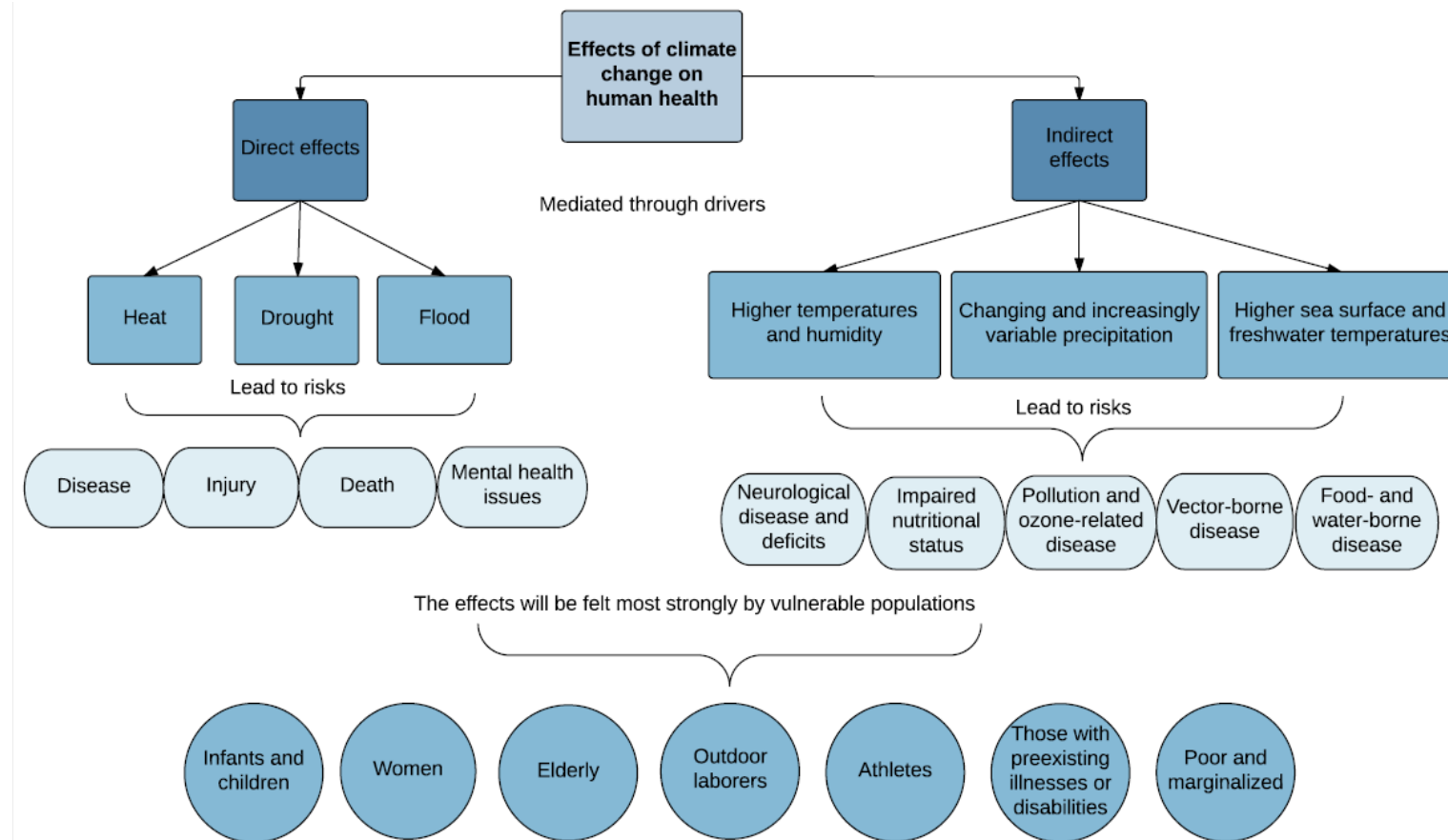
Figure 3.1 Effects of climate change on human health
