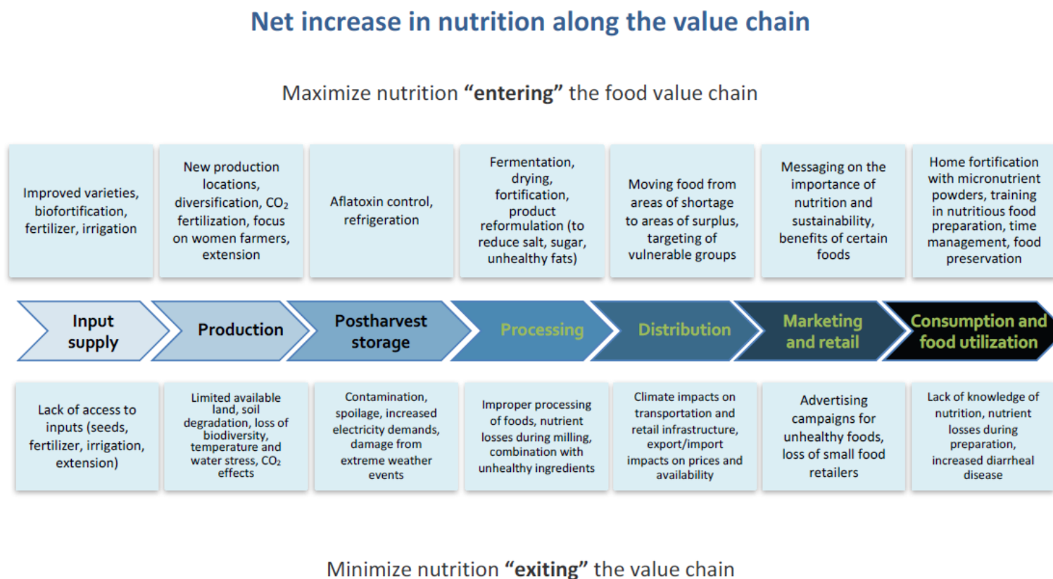
Figure 1.1 Climate change and nutrition entry and exit points in the food value chain
