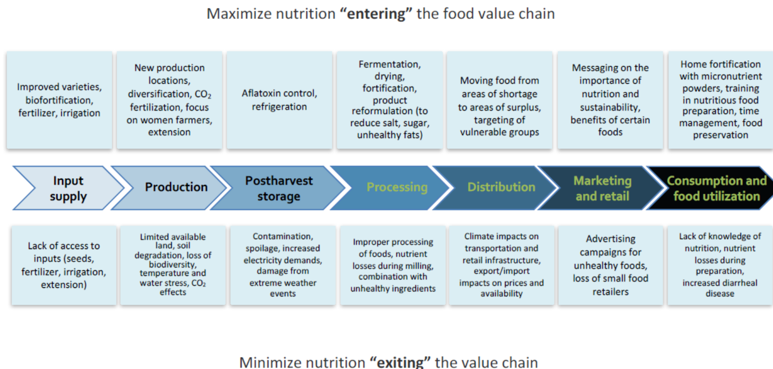
Figure 6.1 A climate-smart and nutrition-sensitive food value chain
